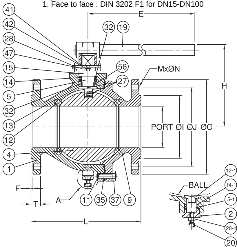
A VIEW SUPPORT BALL DESIGN 10" 12"
