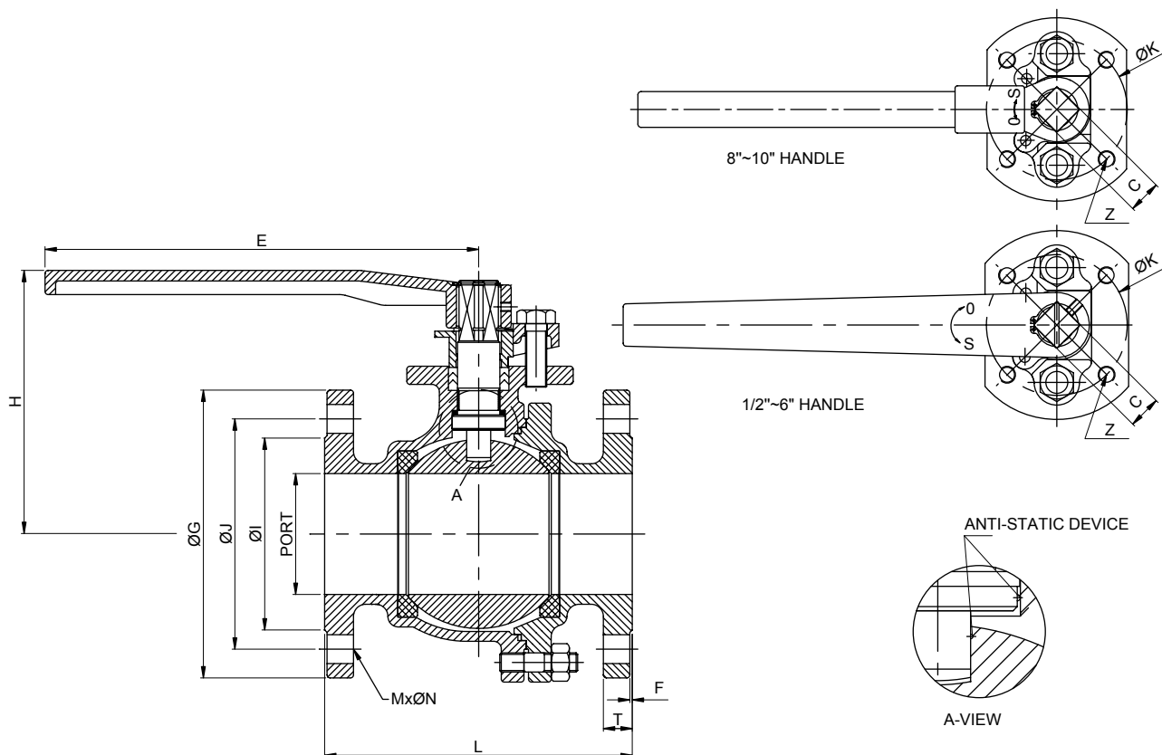
Fig No: MD-52-150 Full Bore 1/2" ~ 10" DN15 ~ DN250
