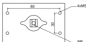
DETAIL "X"
