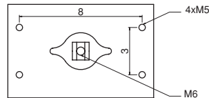
DETAIL "X"
