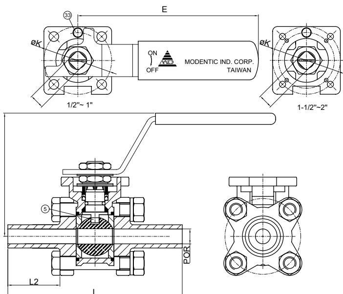
US/3A Dimensioned valves in mm
